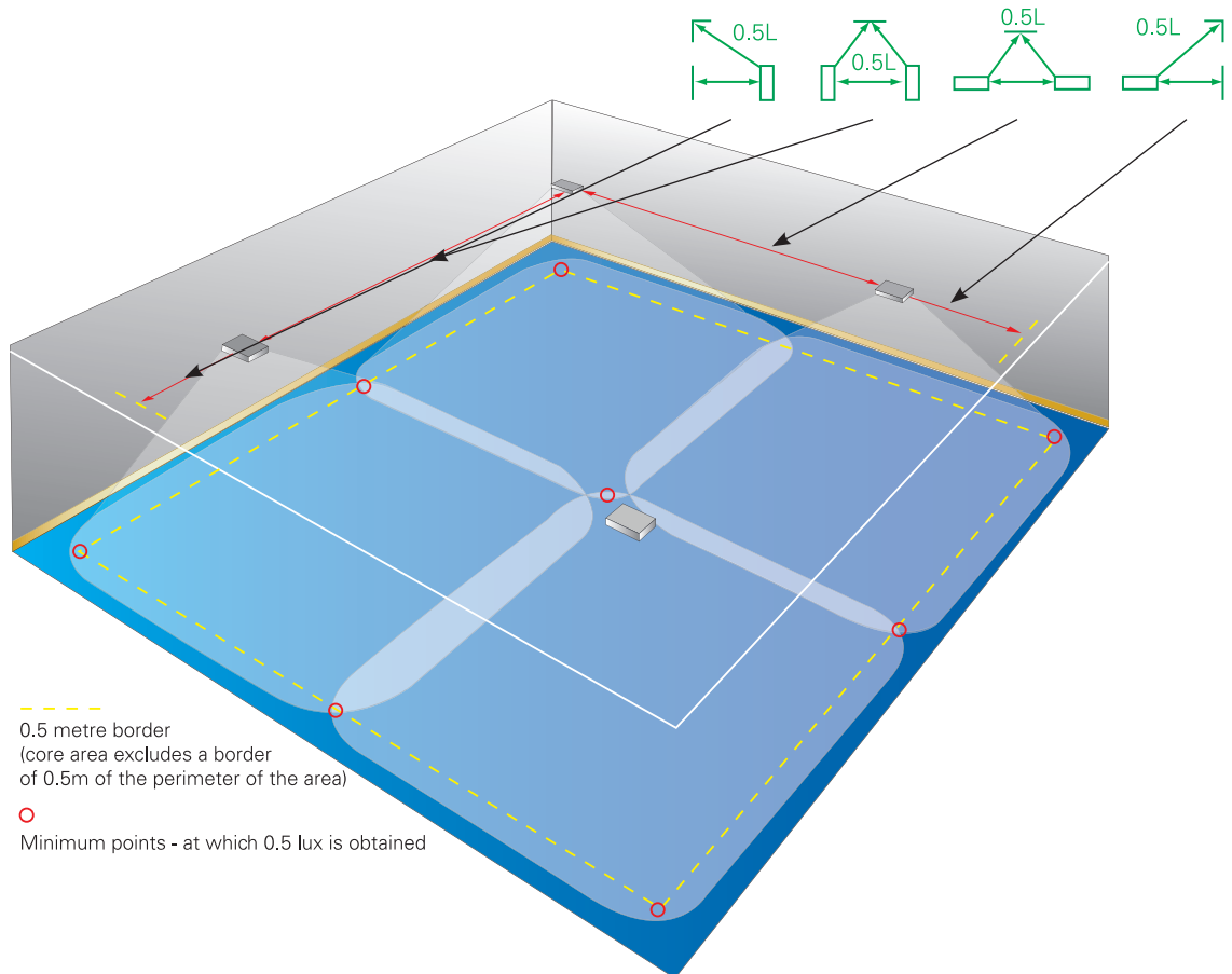
Luminaire spacing in open (anti-panic) core areas
